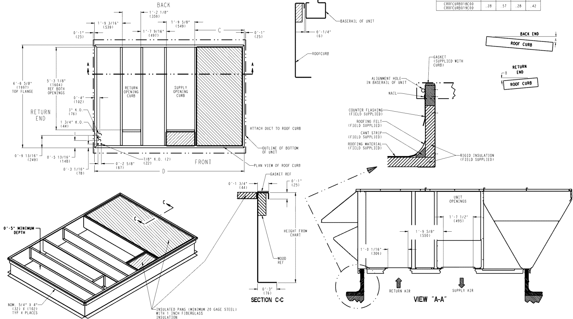
Fig. 1 — Roof Curb Details
