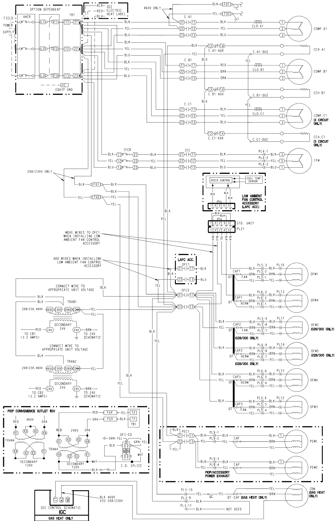
Fig. 41 — Power Schematic
