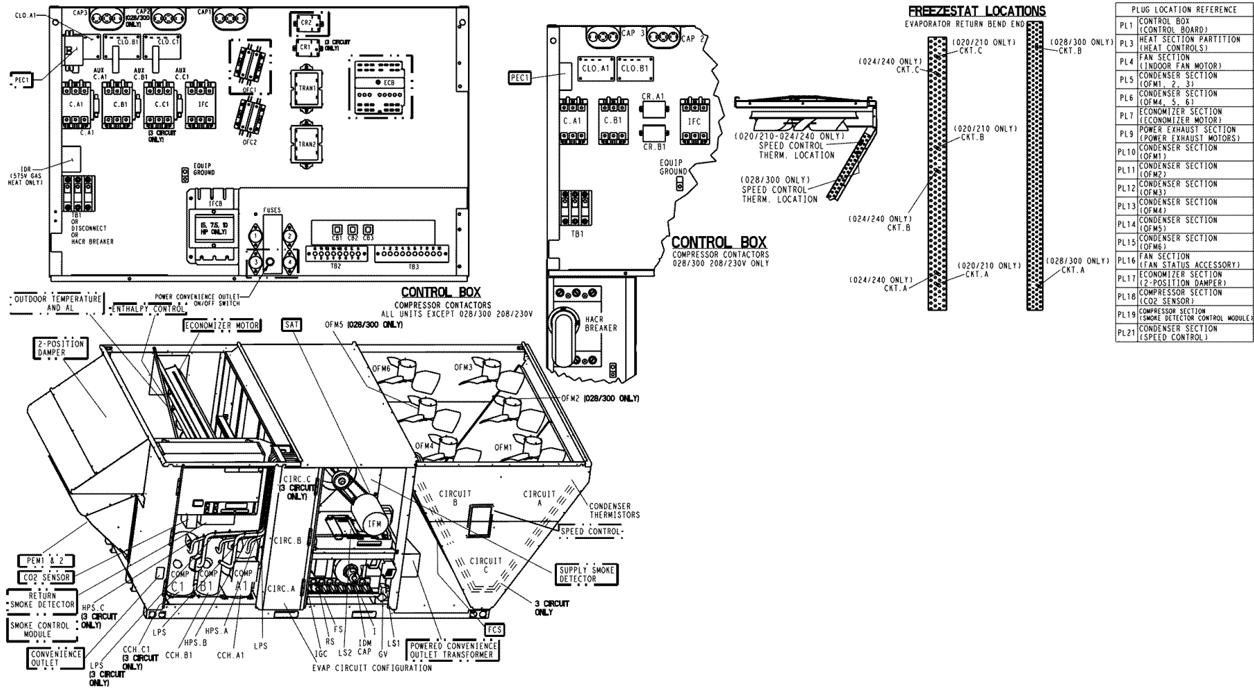
Fig. 42 — Component Arrangement
