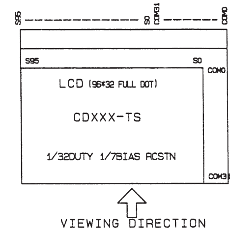
LCD-TAB Connection
