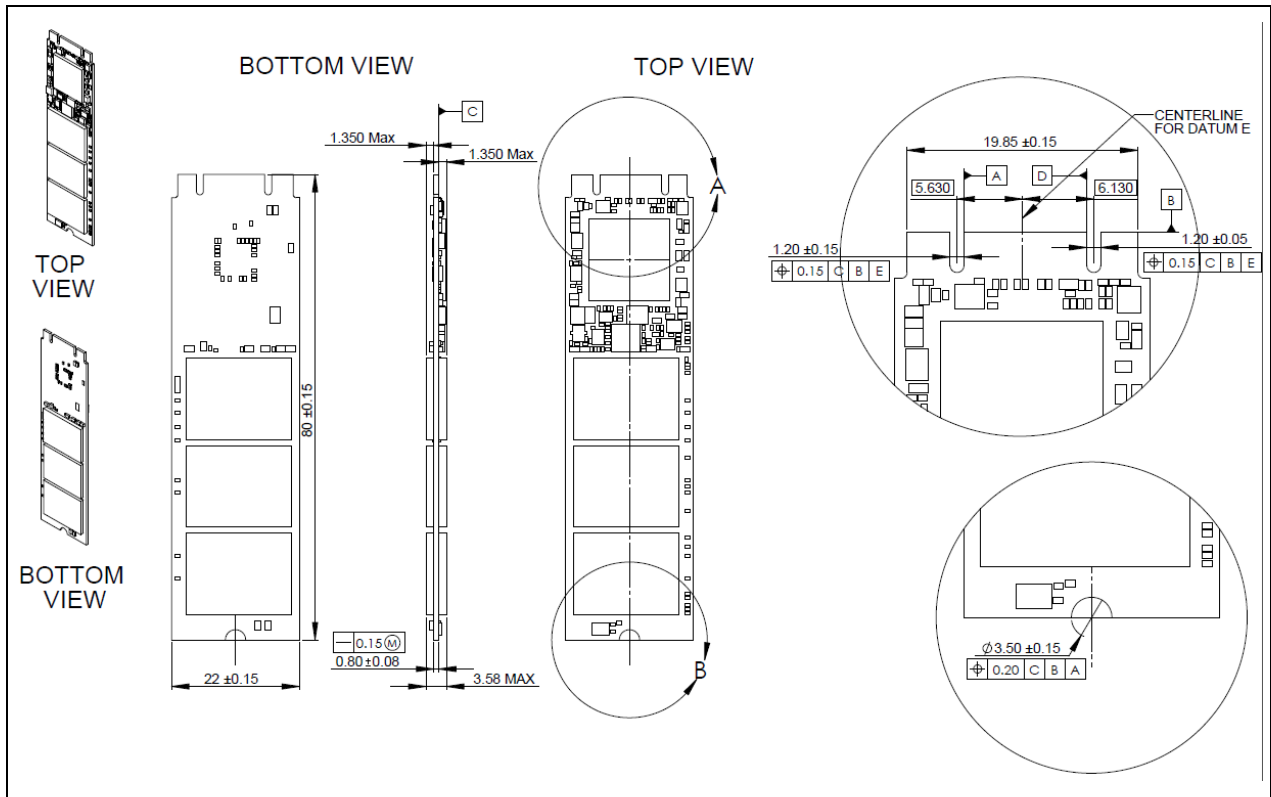
Figure 1: Dimensions for 80 mm double-sided M.2 Form Factor (2280-D2-B-M) 120 GB and 360 GB
