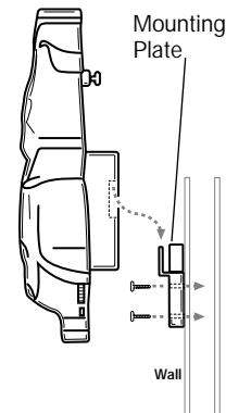
4 Mounting Screws
