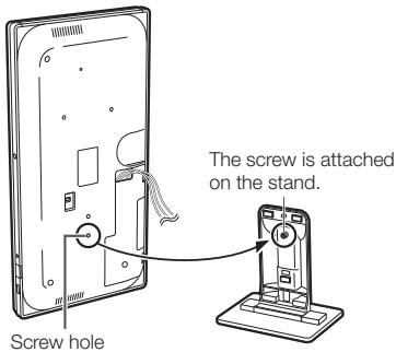
Screw hole
