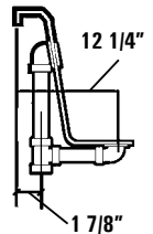
Rough-In Plumbing Measurements
