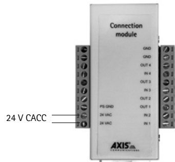
AXIS 231D+/232D+ Module de raccordement
