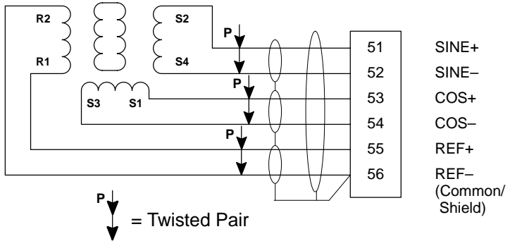
Figure 4-2 Resolver Connections
