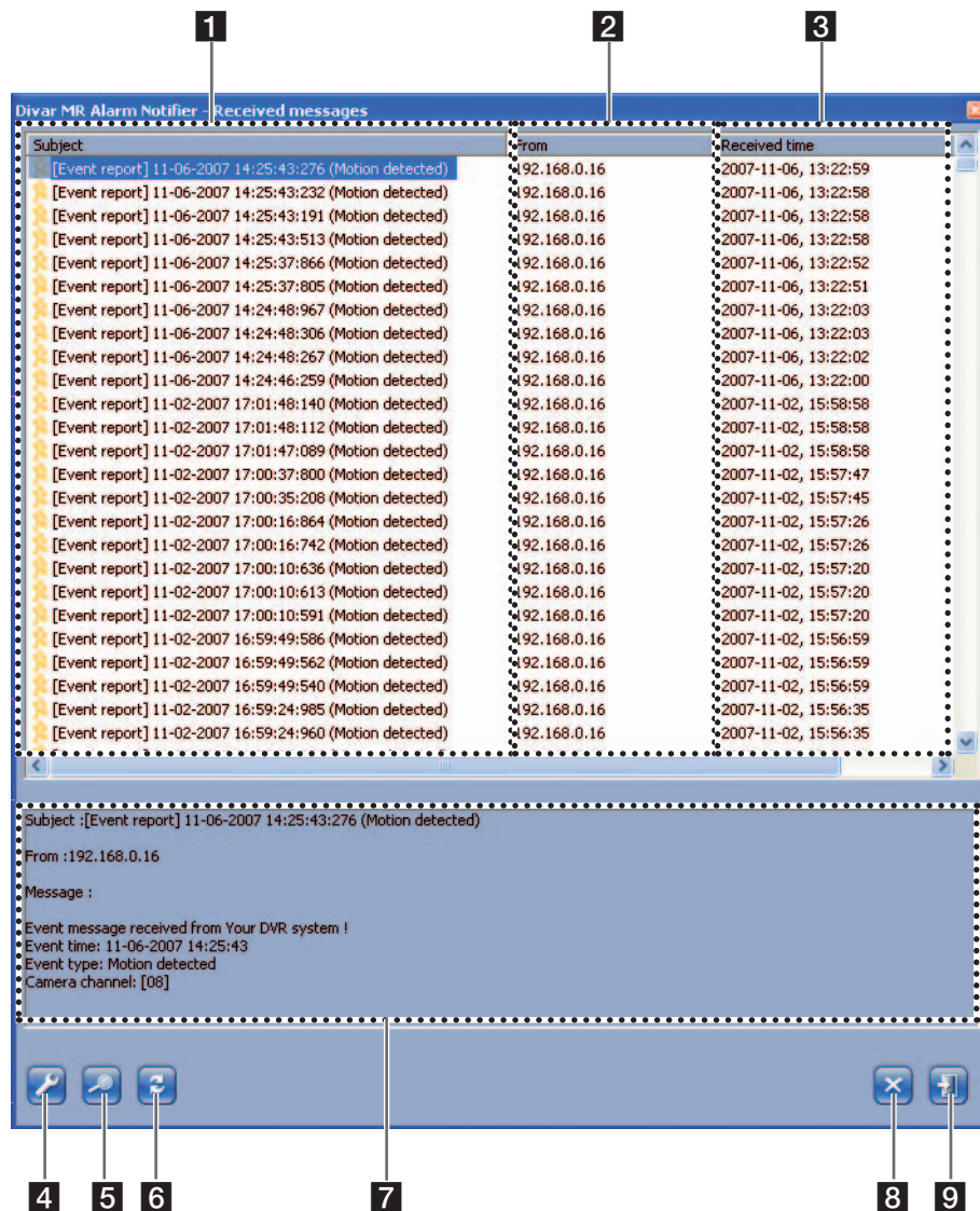
Figure 7.3 Main Screen of Emergency Agent
