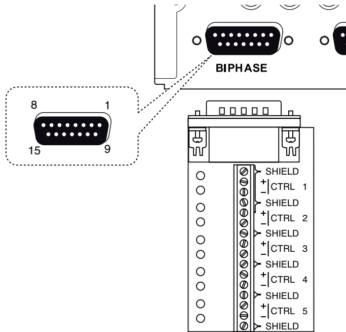
Figure 3.3 Biphase port connector
