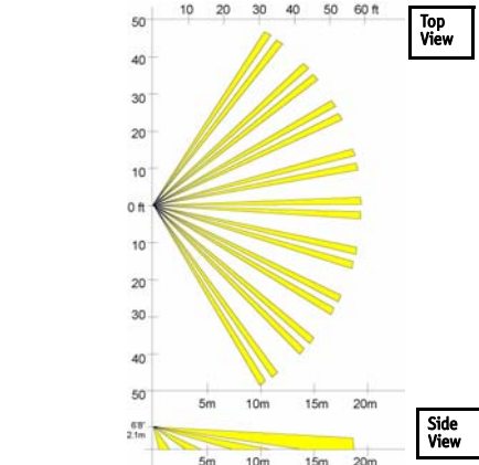
Fig. 3 ES1260 Zone Map
