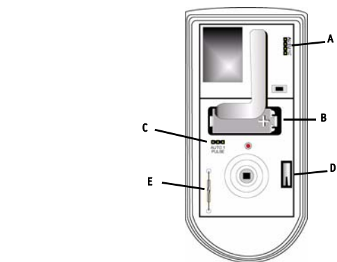
Fig. 2 ES1260 Components
