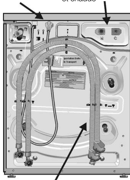
Tuyau AQUASTOP
