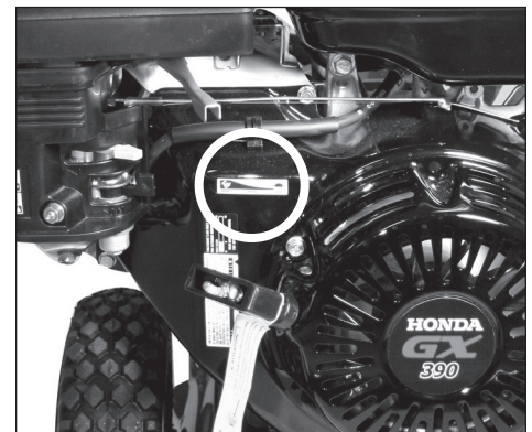
Figure 10 - Throttle
