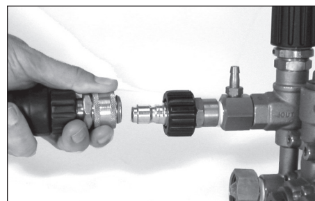
Figure 5 - Connect high pressure hose to pump
