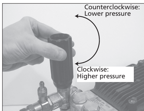
Figure 11 - Camshaft pump pressure adjustment
