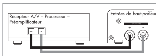
Figure 1 POLARITÉ
