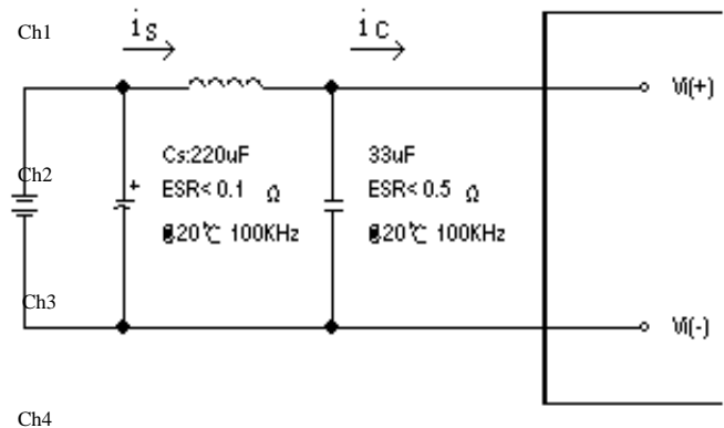
Figure 12: Test set-up diagram showing measurement points for Input Terminal Ripple Current and Input Reflected Ripple Current.
