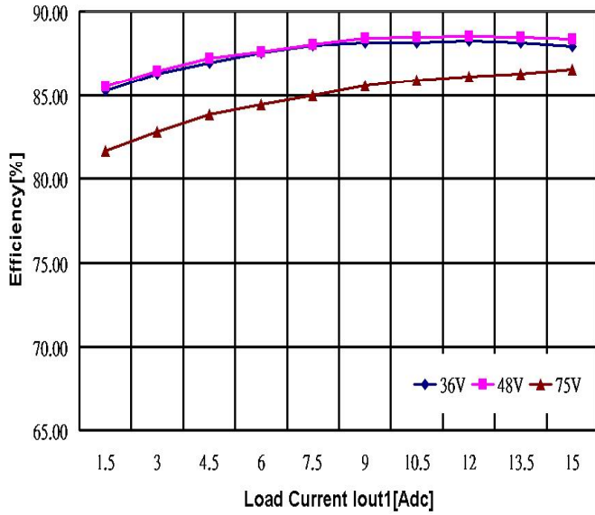
Figure 1: Efficiency vs. load current Iout1 for minimum, nominal, and maximum input voltage at 25°C, for Iout2=7.5A.
