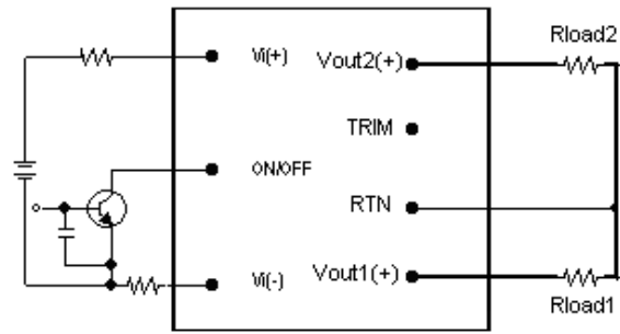
Figure 19: Remote on/off implementation
