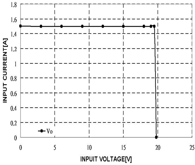
Figure 17: Output voltage vs. load current I_{out1} showing typical current limit curves and converter shutdown points.
