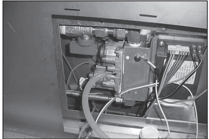
Figure 6.5 Connect Manometer
